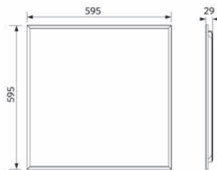
LEDPanelS-P6 Sq595
