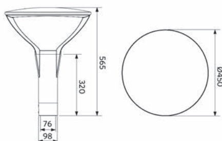
LEDPostTop-Pn D76
