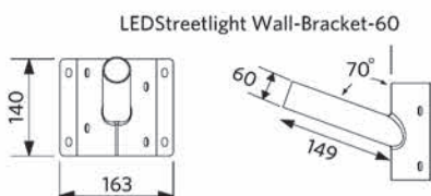
LEDStreetlight Wall-Bracket-60
