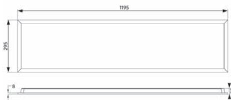
LEDPanelS-B3 Re295-32W
