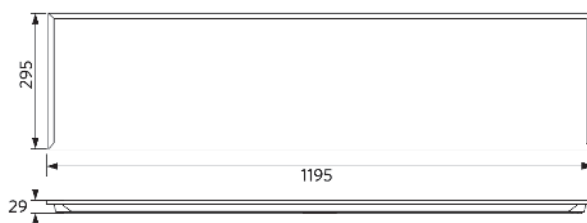
LEDPanelS-P6 Re295
