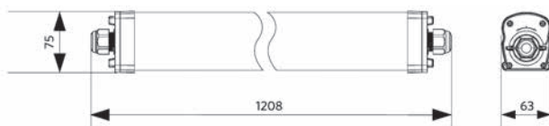
LEDWaterproof-P4 L1208
