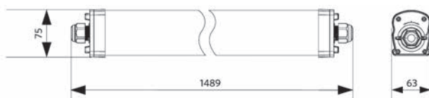
LEDWaterproof-P4 L1489
