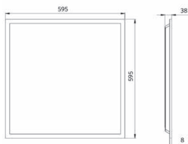
LEDPanelS-B3 Sq595-32W
