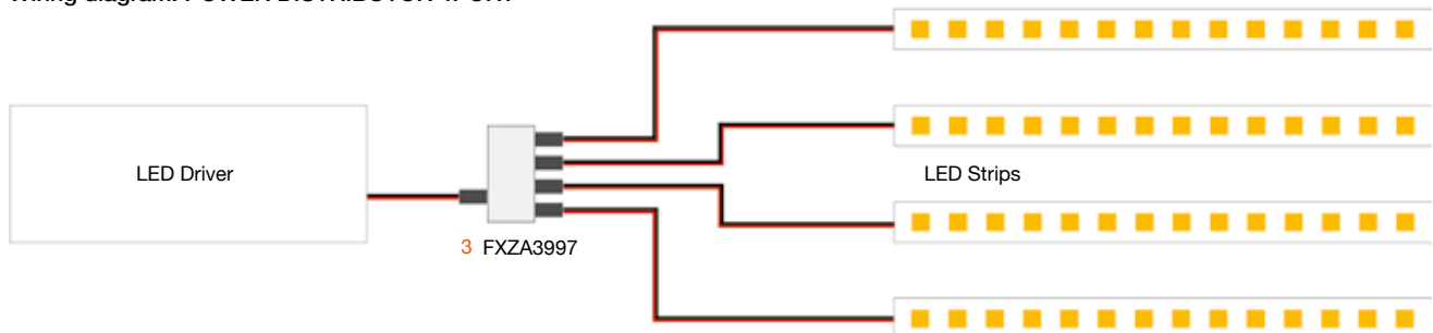
Wiring diagram: POWER DISTRIBUTOR 4PORT
