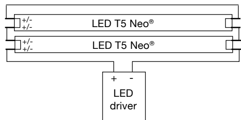
Connection example LED T5 Neo® 2-lamp:
