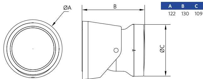
560006000900 - LEDSmart-Sensor IP65-Base-Module
