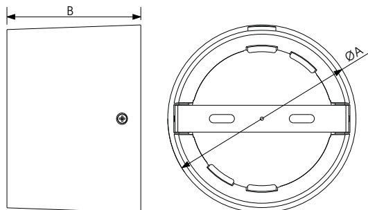
560098000600 - LEDSmart-Sensor Surface-Module-WH
