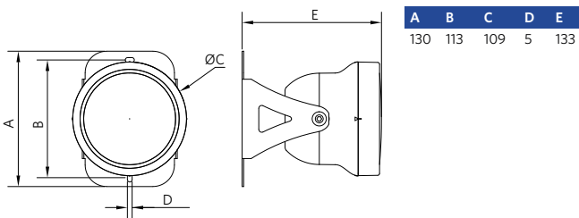
560006001000 - LEDSmart-Sensor IP65-Module
