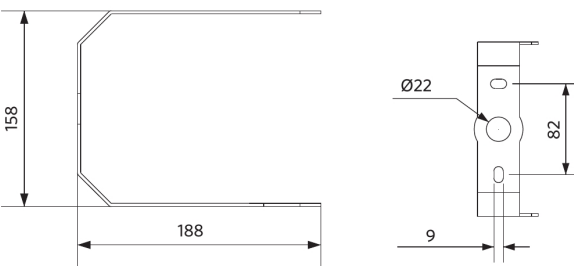
LEDHighbay-P5 Bracket-D330
