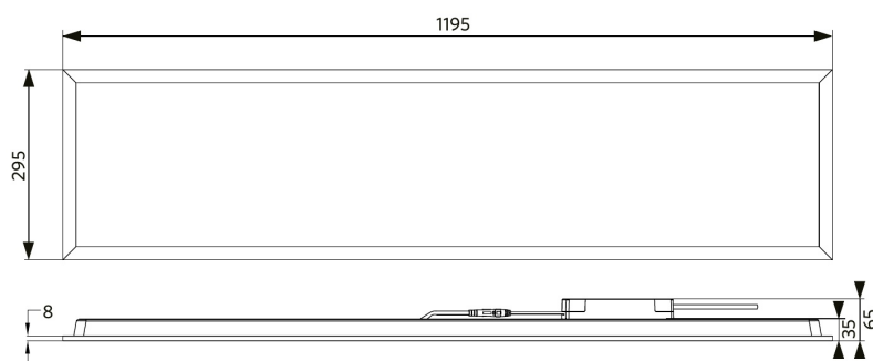
LEDPanelS-E3 Re295-32W
