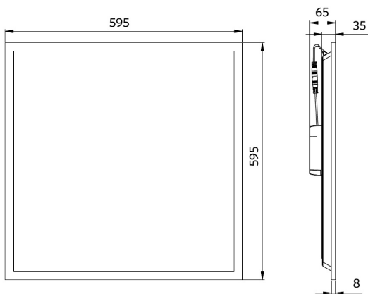
LEDPanelRc-S-B2 Re295-32W
