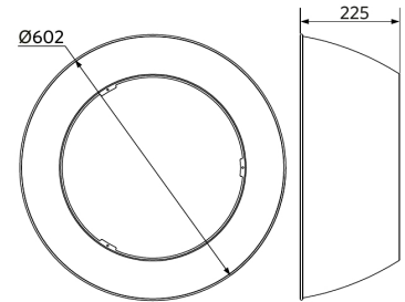
LEDHighbay-E2 Reflector-Rd602
