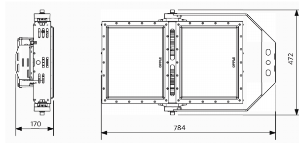
LEDfloodHO-P-620W (+MountingKit-2Mod)
