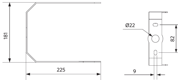
LEDHighbay-P5 Bracket-D420
