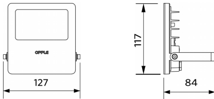
LEDflood-E2 Re127
