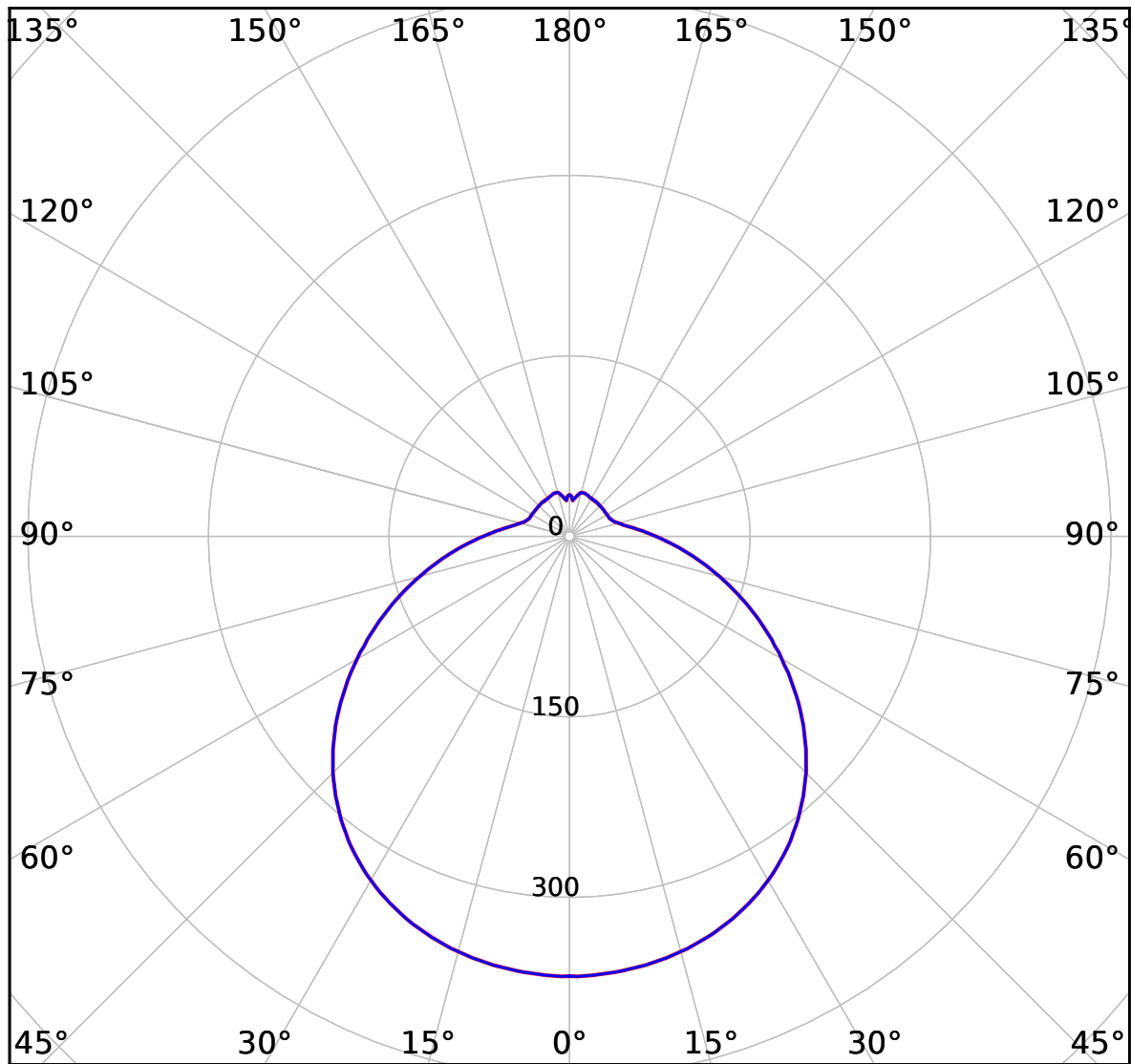
cd 1580 lm — C0-C180 — C90-C270
