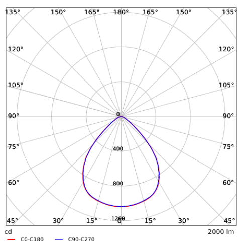
Polar Diagram_140046187
